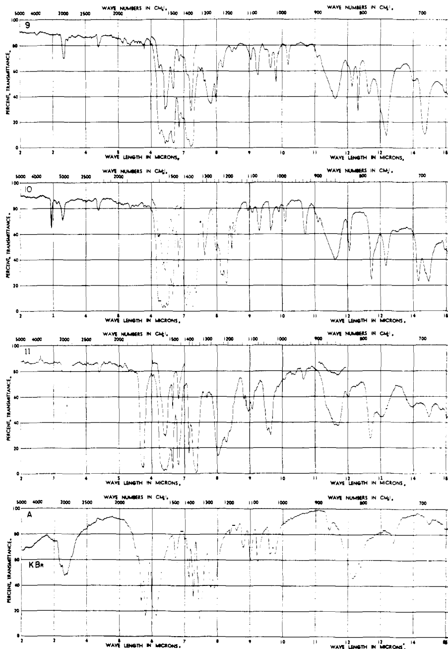
Fig. 3.—Solution spectra: 9, 2-bromomethyl-4,6-bis-(diphenylamino)- s -triazine; 10, N -phenyl-2-phenyl-6-phenoxy-4-amino- s -triazine; 11, 2-dicarboethoxyphenylmethyl-4,6-dimethoxy- s -triazine; KBr spectra: A, 2-dicarboethoxymethyl-4,6-dihydroxy- s -triazine.
